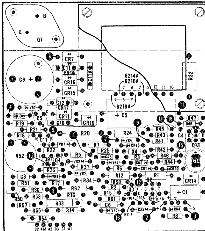
Figure A-2. Model 6216A, Component Location Diagram
